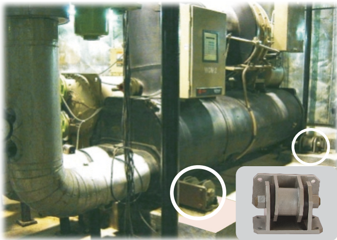
DESIGN OF ALL DIRECTIONAL SEISMIC SNUBBER FOR 4 NOS. TRANE CENTRIFUGAL WATER CHILLER (U.S.A.) (weighing 8 Tonnes each) to protect against Earthquakes at Indira Gandhi National Centre for Arts, New Delhi ▲
